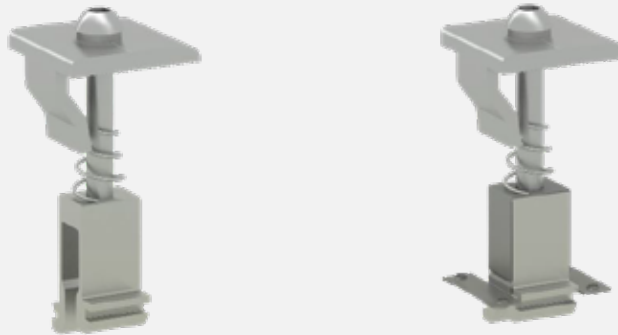
Universal Clamp for Frame Height 30-46mm
