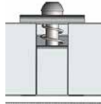
Used as Inter Clamp
