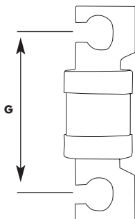
BS88: 1988 Part 5 Dimensions in mm
