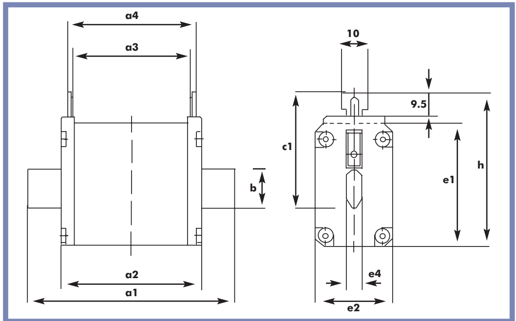
Dimensions size 000 to size 4a
