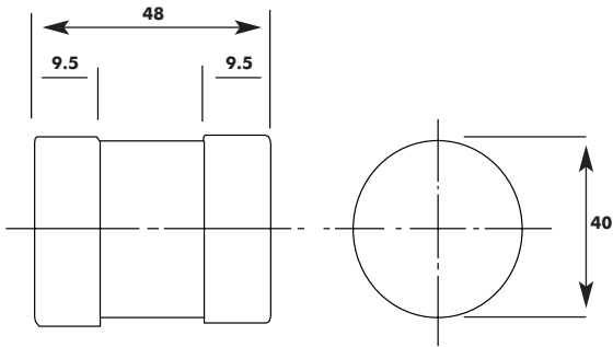
BS88: 1988 Part 5 Dimensions in mm
