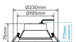
Remote Driver 127 x 43 x 28mm
