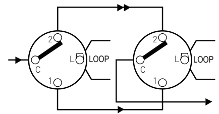
MULTIWAY SWITCHING 2 SWITCHES
