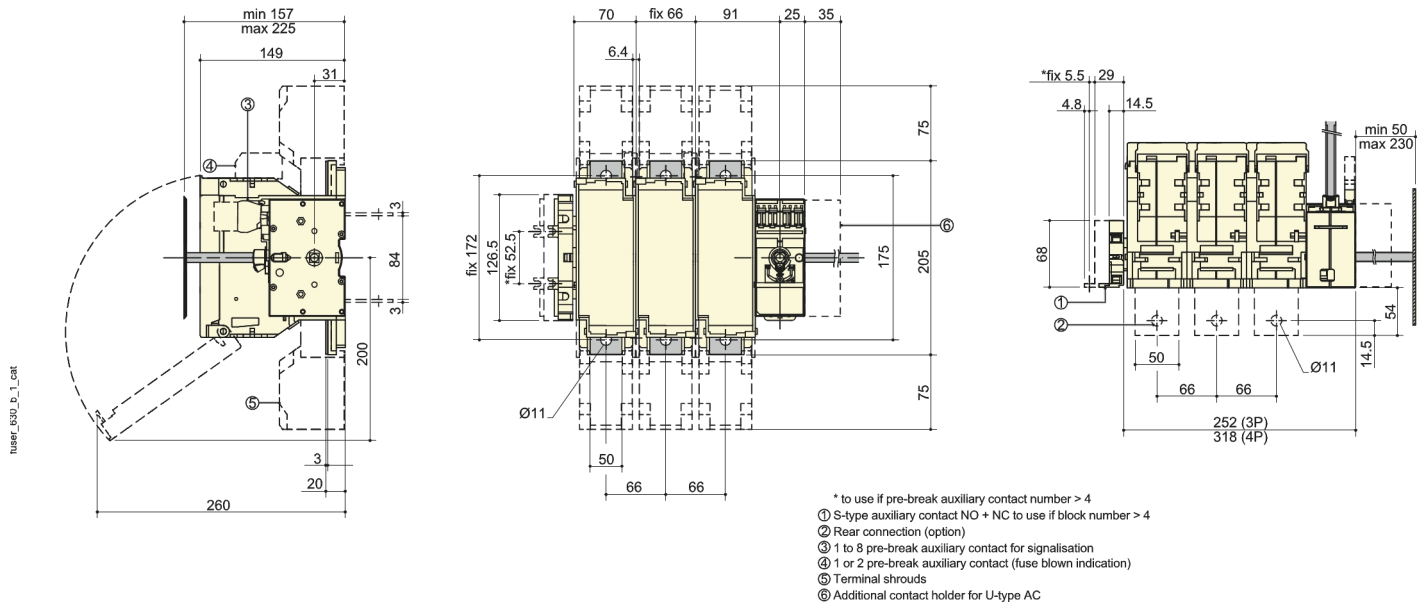
Dimension Diagram
