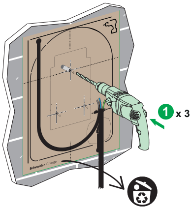
Cable entry from the bottom
