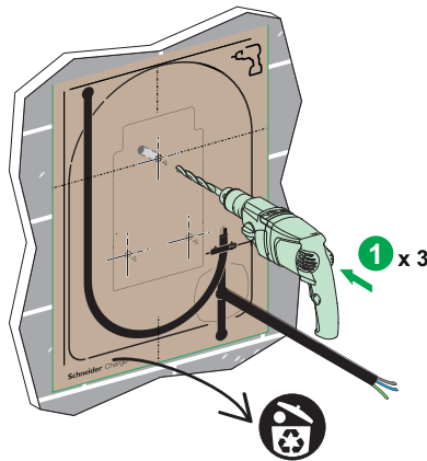
Cable entry through the wall
