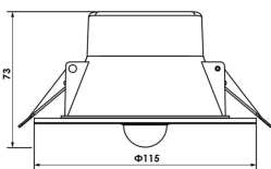
S9062TC-S CUT - OUT 92mm
