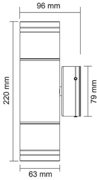
SE7122 GU10
