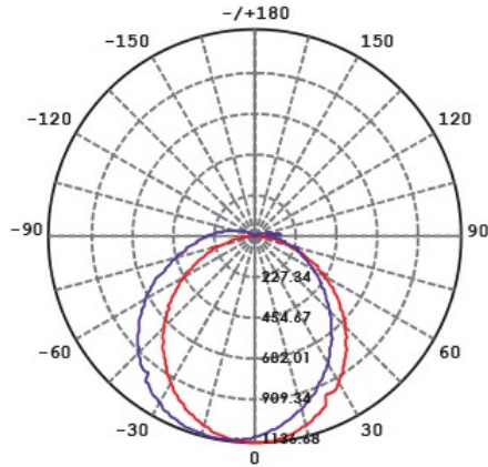
SL9707/120TC at 5700K
