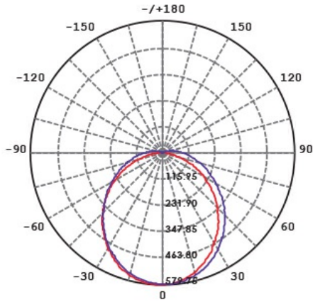
SL9707/60TC at 3000K
